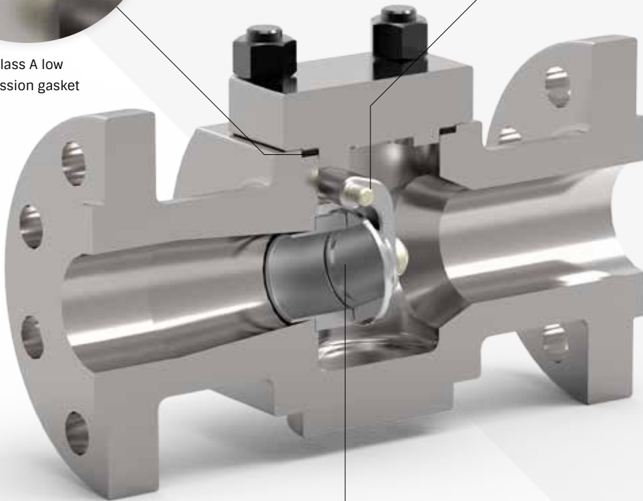
Enclosed hinge pin
