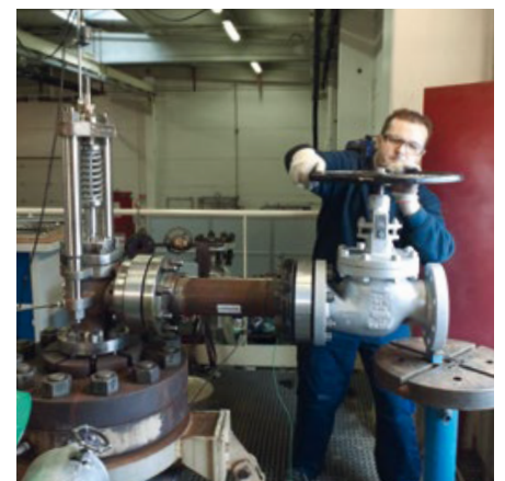
Starsteam® – Back Pressure Test
